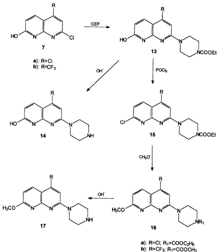
Figure 4. Reagent: CEP, N -carbethoxypiperazine.
