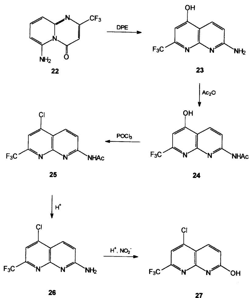
Figure 6. Reagent: DPE, diphenylether.
