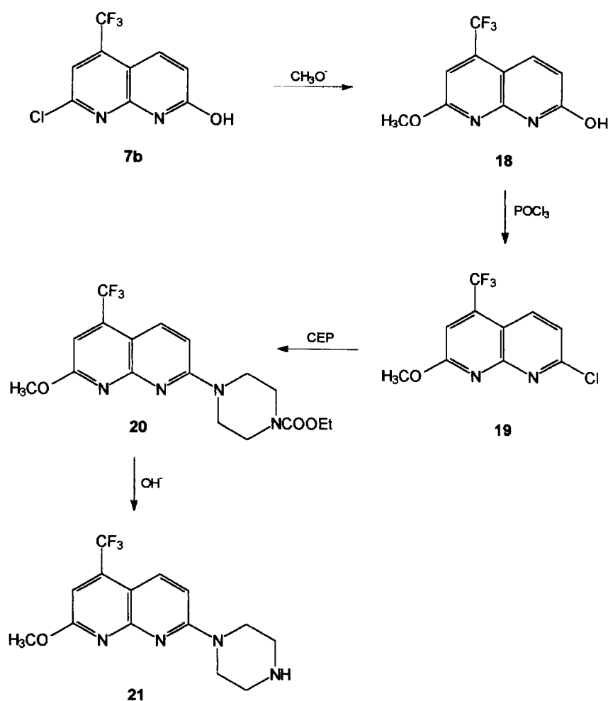
Figure 5. Reagent: CEP, N -carbethoxypiperazine.
