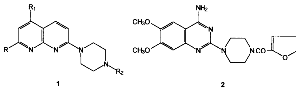
Figure 1. 1,8-Naphthyridine derivatives and Prazosine.
