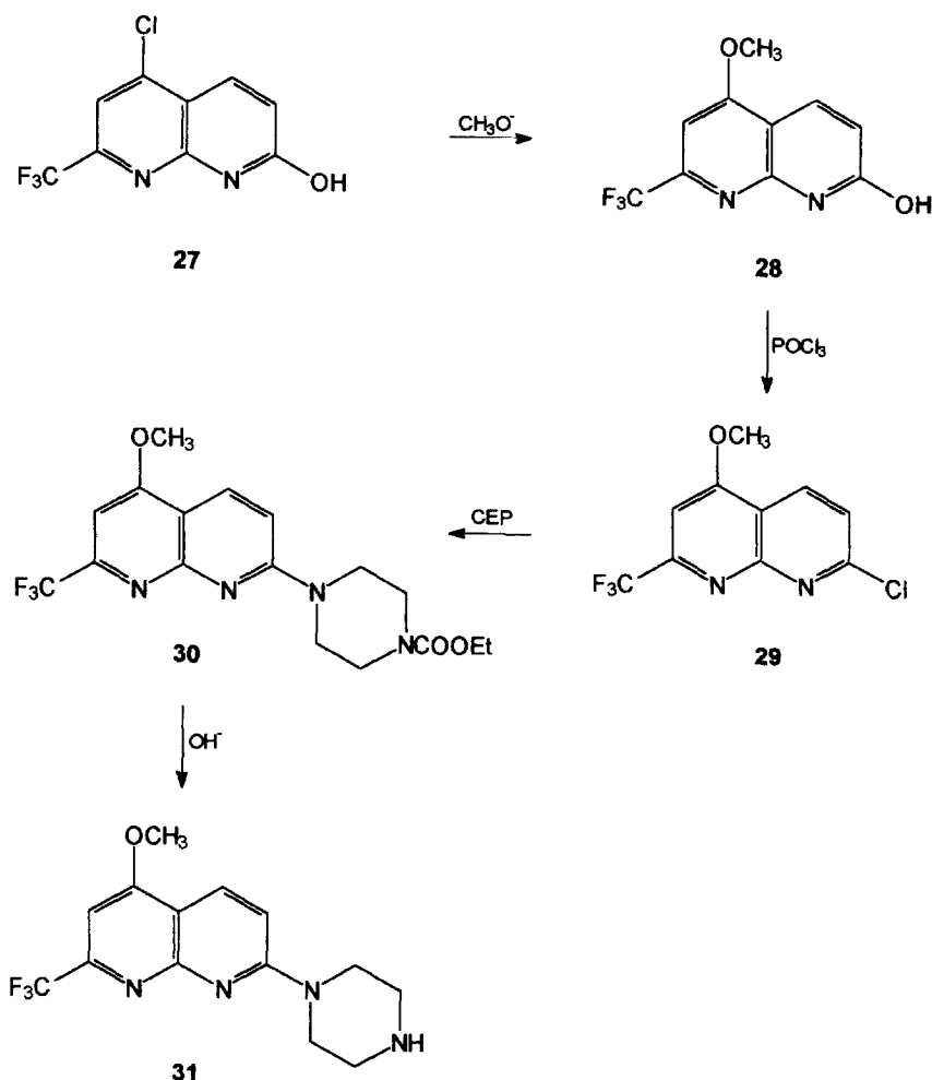
Figure 7. Reagent: CEP, N -carbethoxypiperazine.
