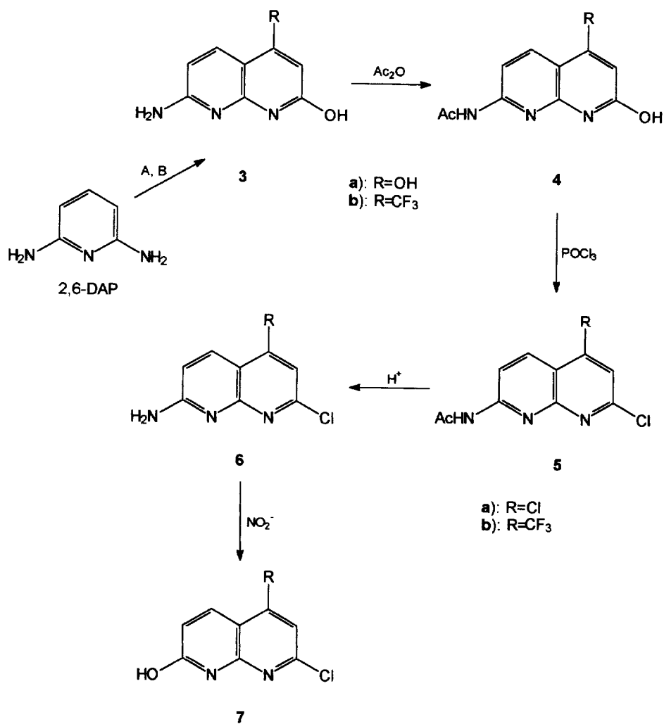
Figure 2. Reagents: A, ethyl malonate; B, ethyl trifluoroacetoacetate.
