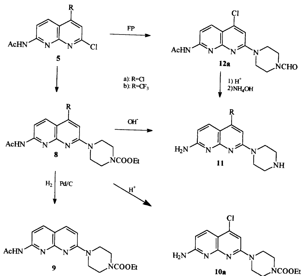
Figure 3. Reagents: FP, formylpiperazine; CEP, N -carbethoxypiperazine.
